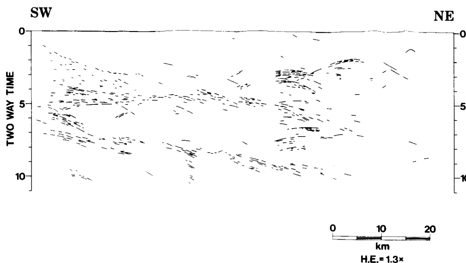
Figure 2. Reflector geometry of Line 1, south-central Vancouver Island (unmigrated).
